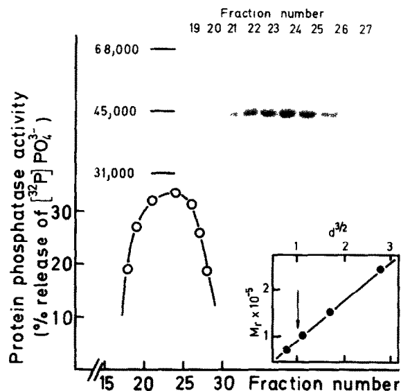
Fig.3. Comparison of the activity of PFK-phosphatase in fractions of a sucrose density gradient with the corresponding protein pattern obtained by SDS polyacrylamide gel electrophoresis. Experimental details are given in section 2. PFK-phosphatase sedimented in the sucrose gradient with about M_{r(app.)} 90000 (see inset). Aliquots (60 \mu l) of the gradient fractions containing PFK-phosphatase activity were directly used for SDS polyacrylamide electrophoresis, where the protein migrated with M_{r(app.)} 44500. Marker proteins for the SDS electrophoresis: bovine serum albumin ( M_r 68000), ovalbumin ( M_r 45000), carbonic anhydrase ( M_r 31000). Inset: plot according to [4] showing the sedimentation behavior of purified phosphatase 2C and PFK-phosphatase (arrow), standard proteins (1, catalase; 2, alcohol dehydrogenase) and control proteins (3, hexokinase; 4, bovine serum albumin) in linear 5–20% sucrose density gradients. The plot represents one out of 7 centrifugation experiments. The molecular mass is given in a logarithmic scale; d, distance from meniscus.
