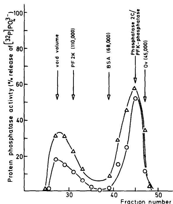
Fig.1. Gel filtration of phosphatase 2C and PFK-phosphatase on Sephadex G-100 was performed as described in section 2. The assays contained 8 mM \text{Mg}^{2+} but no \text{Mn}^{2+} . According to [3] pyruvate kinase was used as substrate for protein phosphatase 2C. The phosphatase 2C/PFK-phosphatase emerging with approx. M_{r(\text{app.})} 55000 was completely dependent on \text{Mg}^{2+} (not shown). ( \nabla — \nabla ) Pyruvate kinase phosphatase, ( \circ — \circ ) 6-phosphofructo-1-kinase phosphatase; PF2K, 6-phosphofructo-2-kinase; BSA, bovine serum albumin; Ov, ovalbumin.
